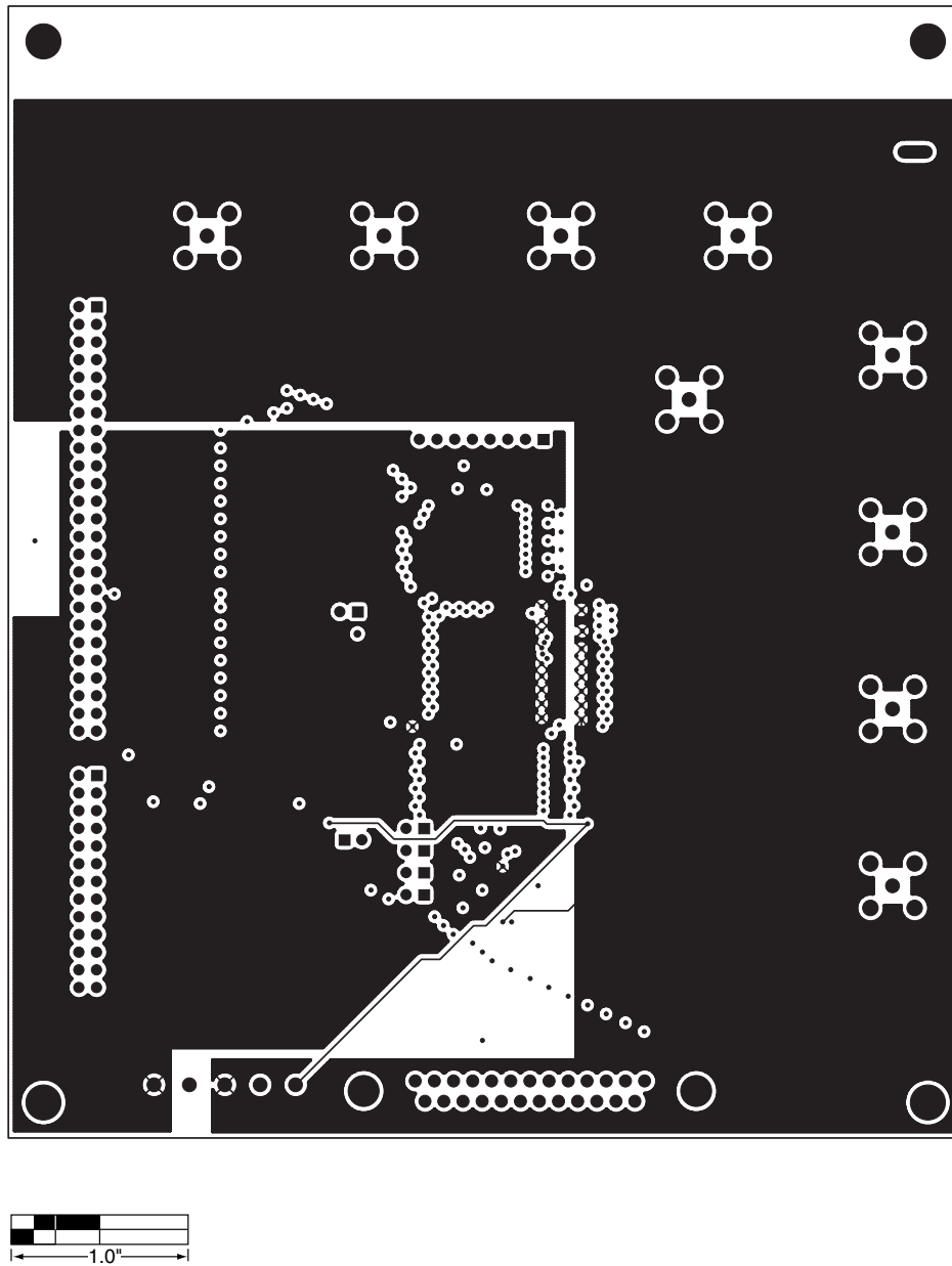
Figure 6. MAX4358 EV Kit PC Board Layout—Layer 3
