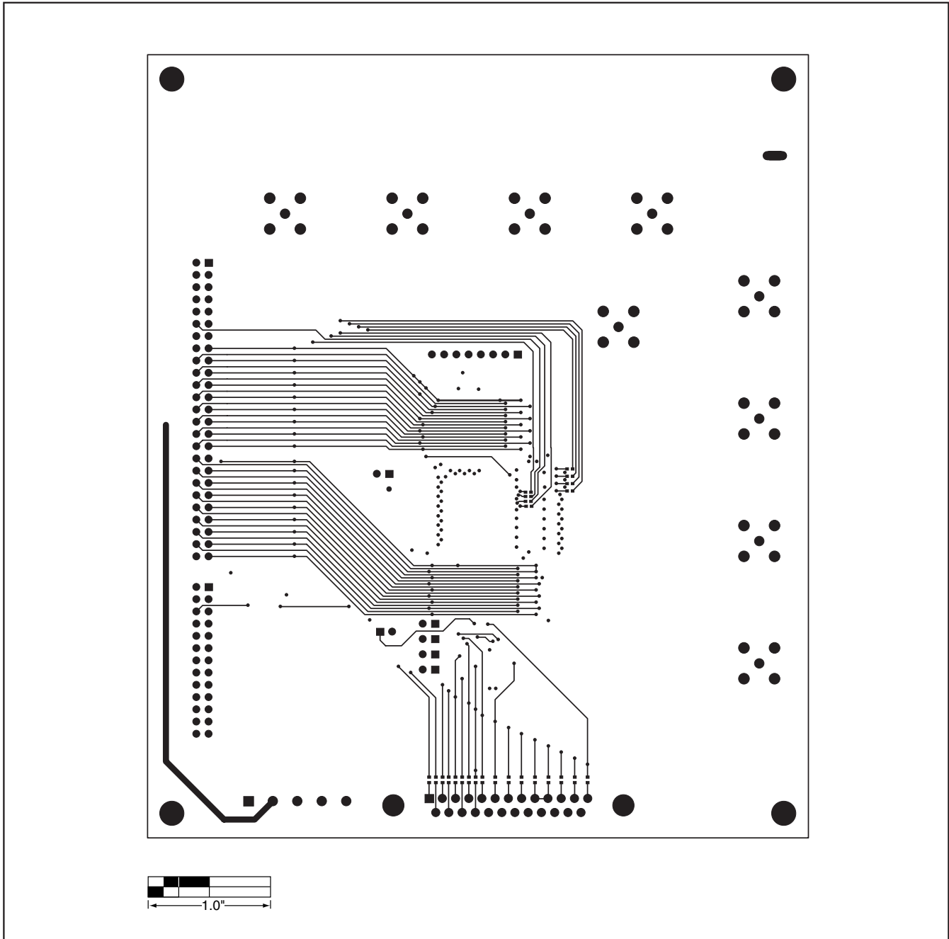
Figure 7. MAX4358 EV Kit PC Board Layout—Layer 4
